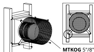
Figure 7.f Installing a MTO, PTO termination heat guard.
