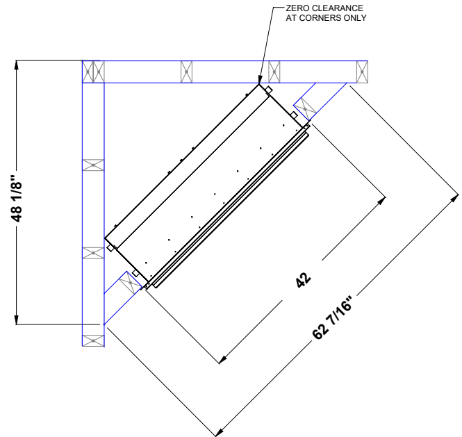
Figure 13 Corner dimensions
