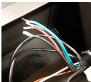
Figure 31 Removal of wire nut
