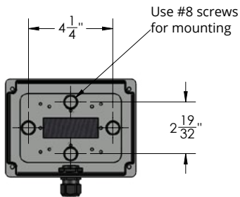
MOUNTING DIMENSIONS (Shown w/o receiver)
