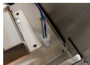
Figure 46 connected power
