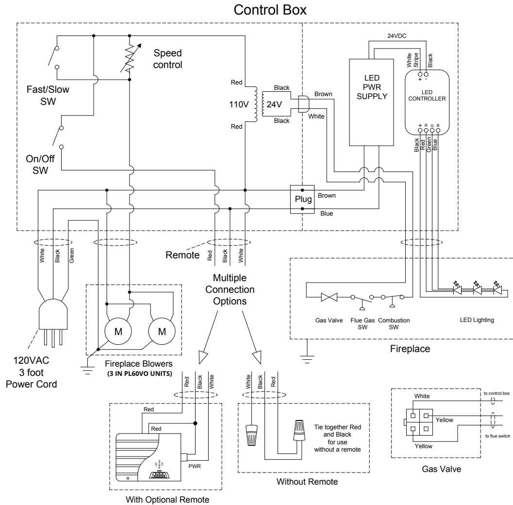
Figure 28 Wiring schematic
