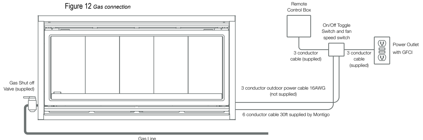
Figure 10 Gas and electrical
