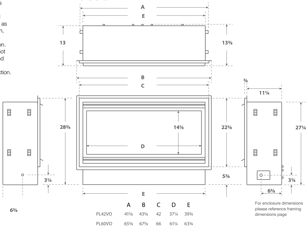
MAHANA Dimensions
