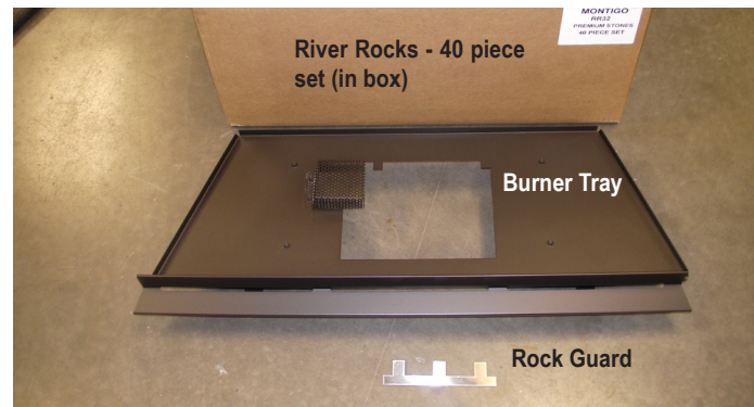
Figure 31. Kit Contents
