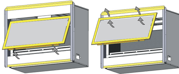
Figure 27g. Removing and installing the glass doors.
