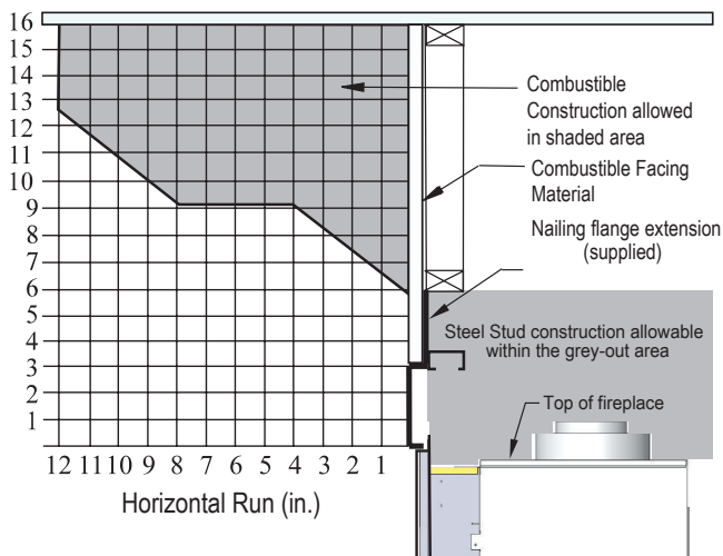
Figure 25a. Combustible mantels and facings, HC34DF* ONLY.
