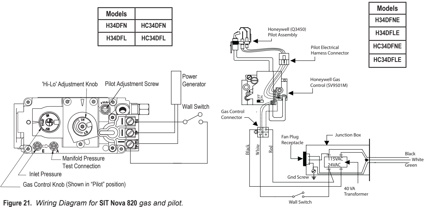
Figure 21. Wiring Diagram for SIT Nova 820 gas and pilot.
