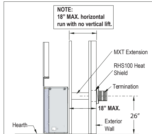
Figure 16a. Straight run, Rear Vented, wall mounted termination for H*34DF*, Figure 16.
