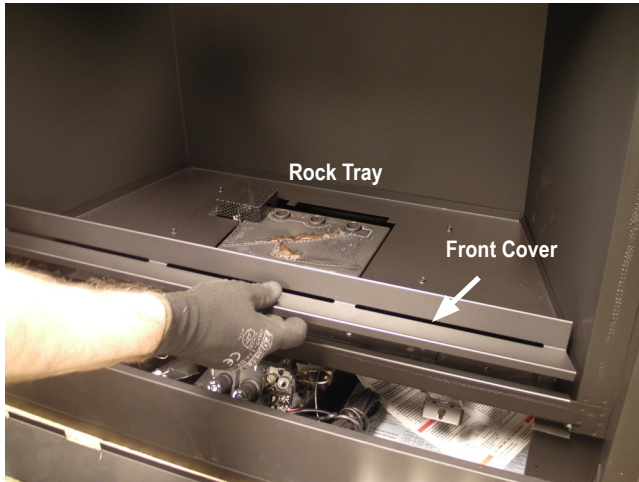
Figure 31c. Burner Tray Front Cover
