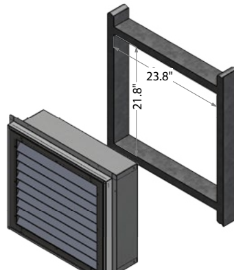
Figure 2.e FGLVBI-10 Framing Dimensions
