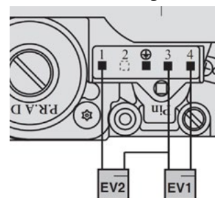
Connection Diagram
