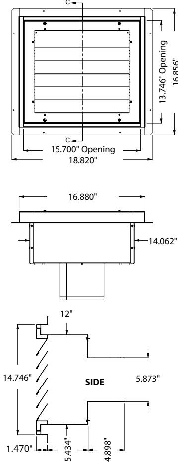
Figure 2. CALVB-06 Dimensions
