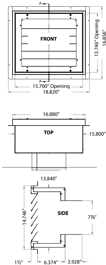
Figure 2. FGLVBI-08 Dimensions
