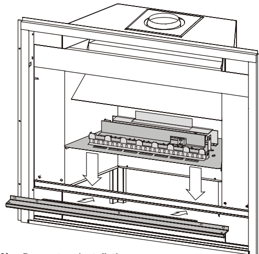
Figure 6b. Burner tray installation.
