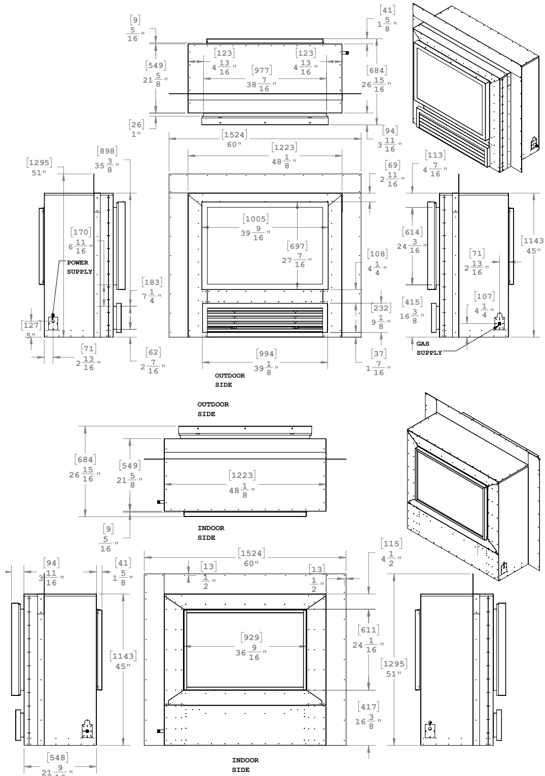
Figure 1. Fireplace dimensions (Tolerance ± 1/8").
