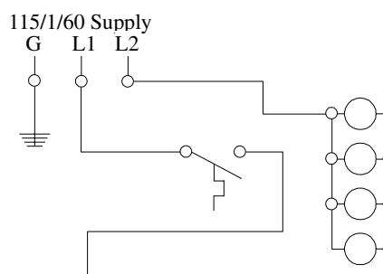
Figure 10 Electrical Connections.
