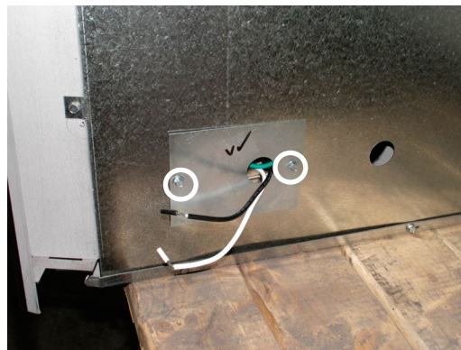
Figure 7 Lead wires that connect to household electrical supply.
