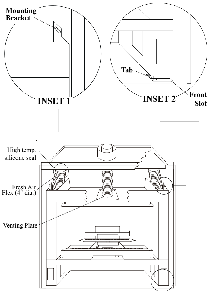
Figure 22. ME38-ODV-2 insert.
