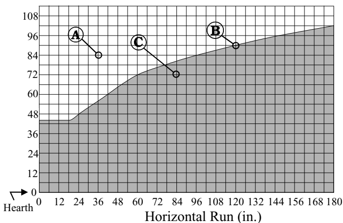
Figure 7. Venting Graph
