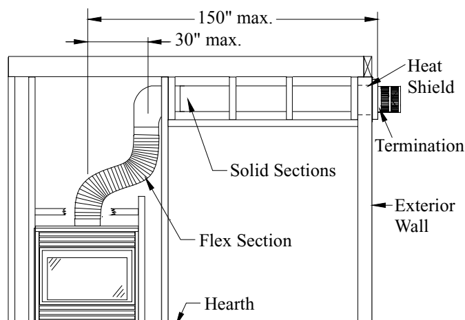
Figure 10. Extended Installation using a combination of solid and flex venting. Use the vent graph to determine your allowable run, then select appropriate components.
