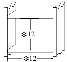
FIGURE 4. VENT TERMINATION FRAMING.
