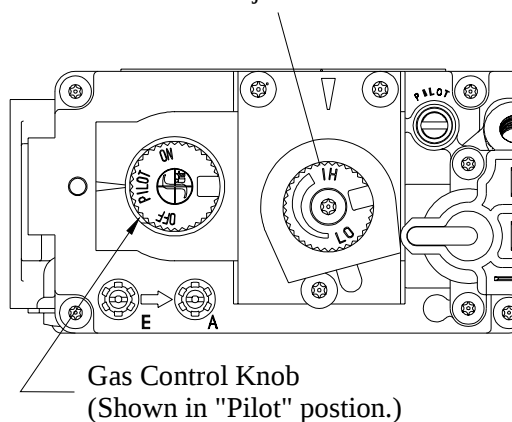
Figure 11. 'Hi-Lo' Adjustment on the ME38-BV's gas valve.
