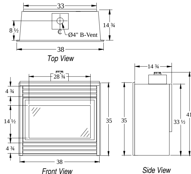
Figure 1. Fireplace dimensions.
