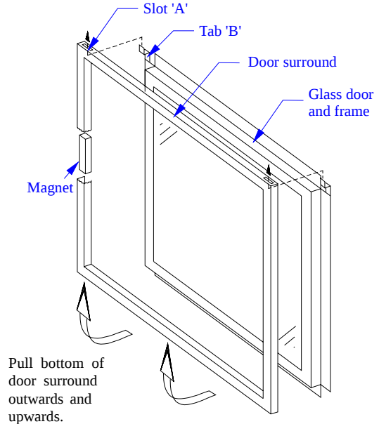
Figure 11a. Removing or installing the door surround.
