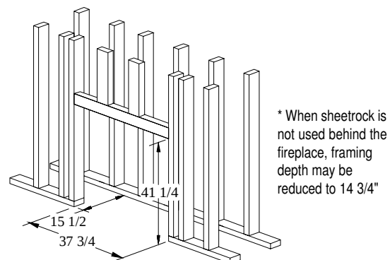
Figure 2. Framing dimensions.
