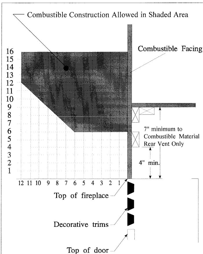
FIGURE 18. COMBUSTIBLE MANTLES & FACINGS
