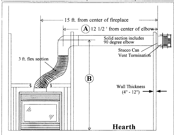
FIGURE 9. EXTENDED 10' SECTION
