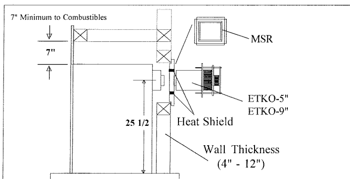
FIGURE 15. STANDARD INSTALLATION
