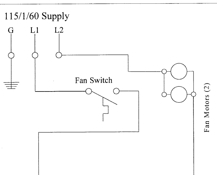
WIRE HARNESS
