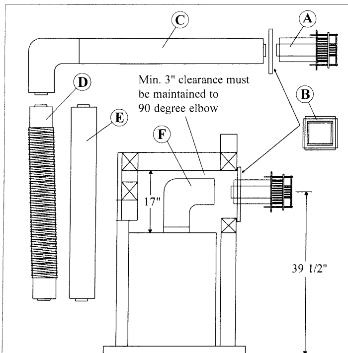
FIGURE 8. TYPICAL INSTALLATIONS.
