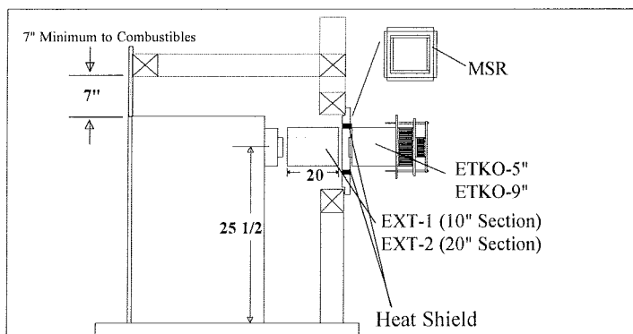
FIGURE 16. EXTENDED INSTALLATION
