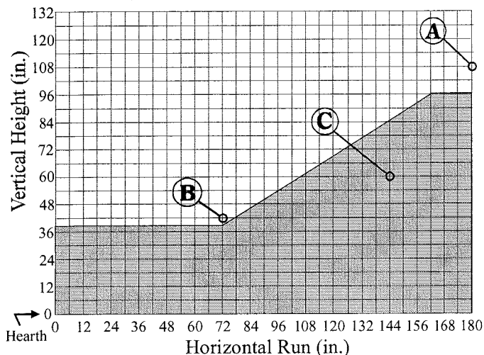
VENTING GRAPH
