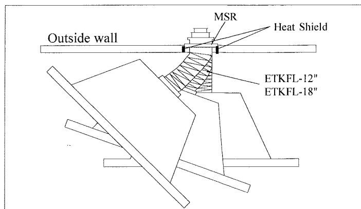
FIGURE 17B. FLEXIBLE INSTALLATION
