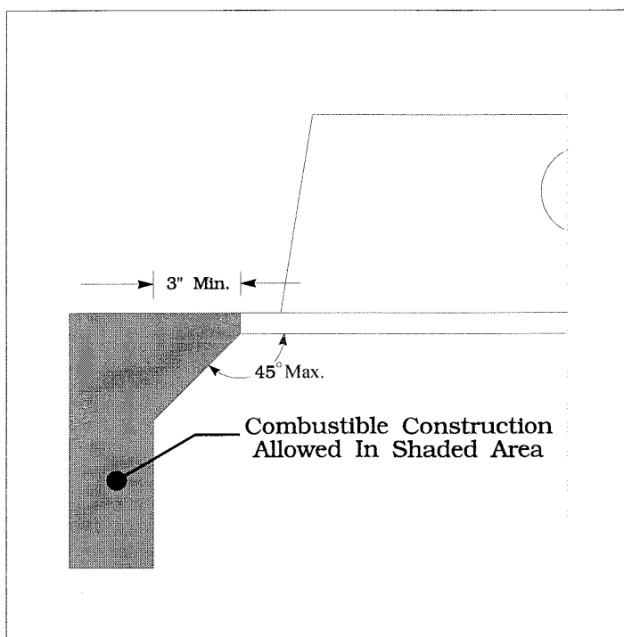
FIGURE 18B. COMBUSTIBLE SURROUNDS
